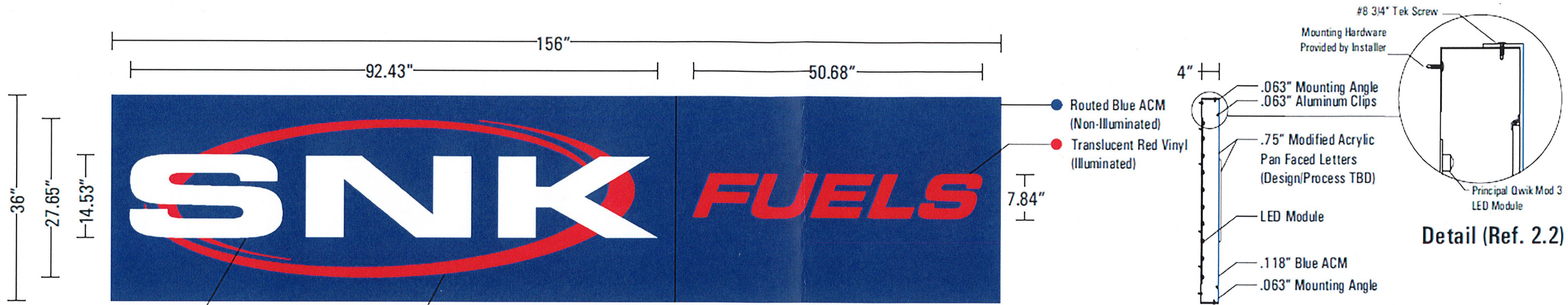
ACM Logo Cabinet (Ref. 2)
