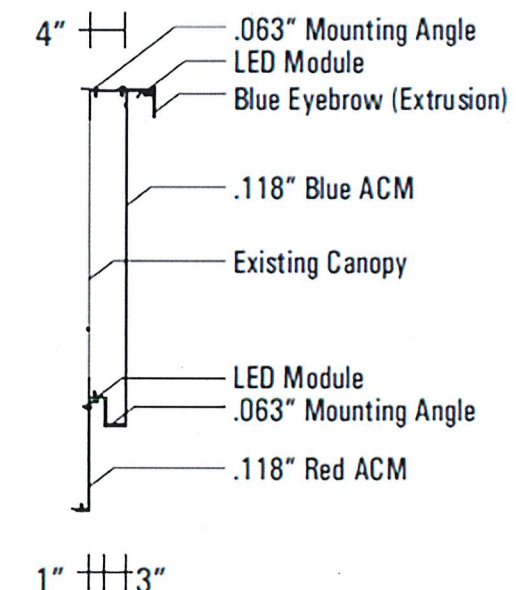
ACM Downlight + Eyebrow Profile (Ref. 3.1)
