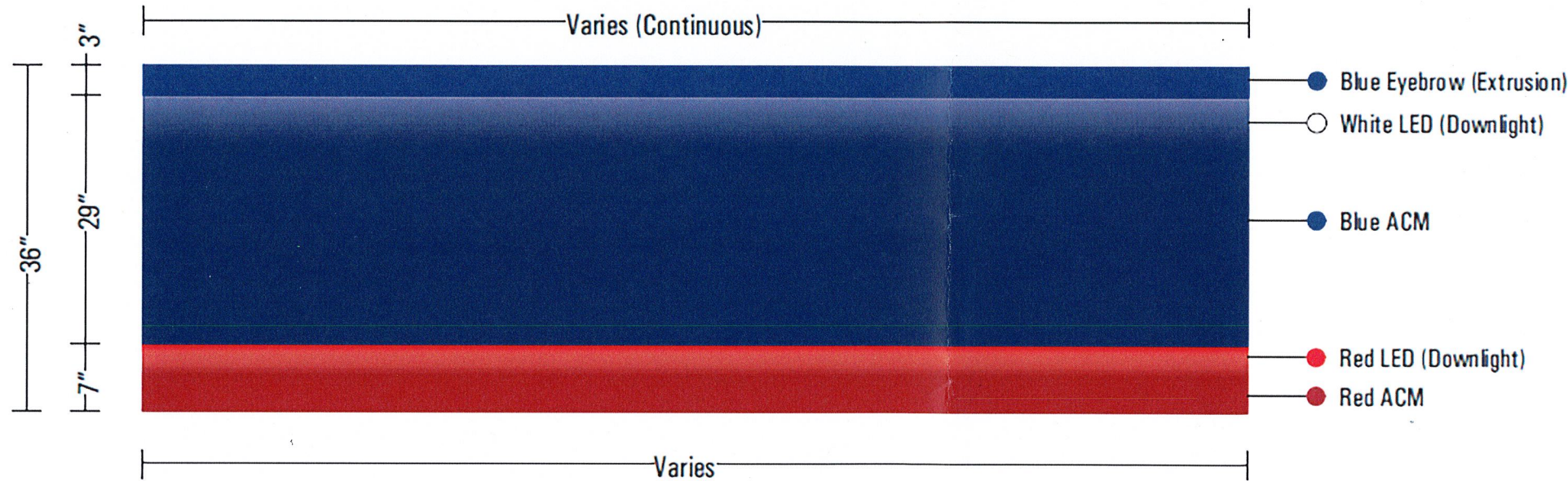
ACM Downlight + Eyebrow (Ref. 3)
