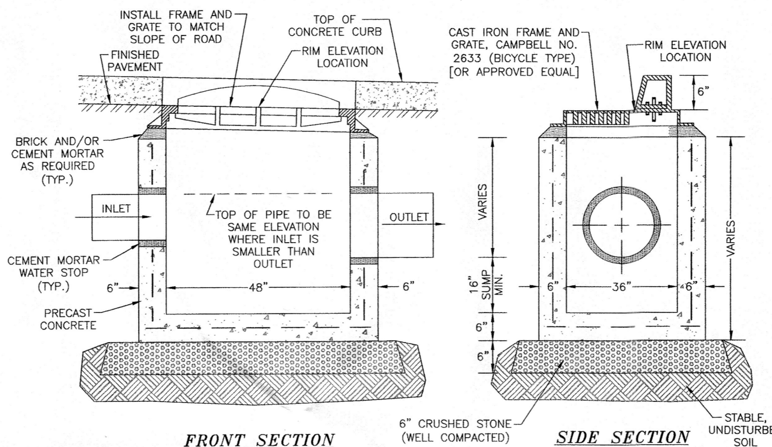
CATCH BASIN DETAIL (CURB INLET) N.T.S.
