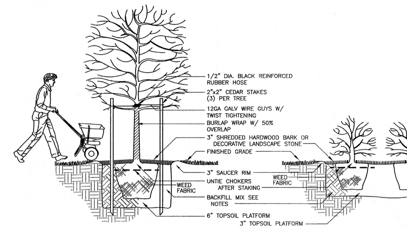
TREE AND SHRUB PLANTING DETAIL N.T.S.
