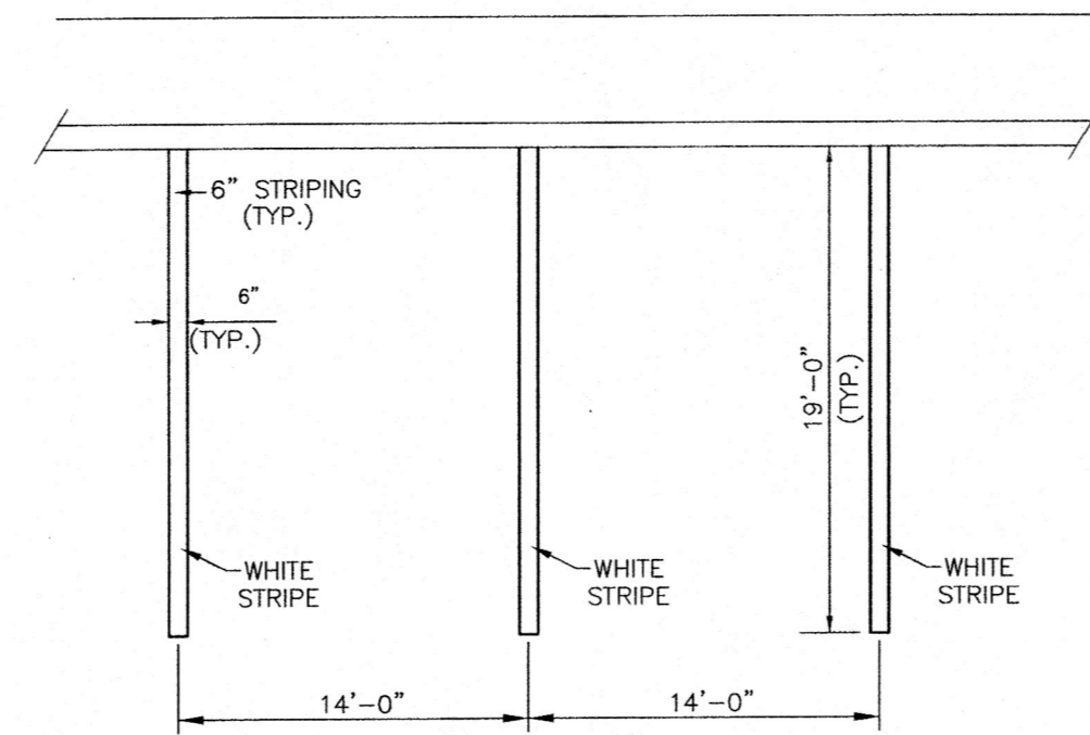
VACUUM SPACE PARKING STRIPING DETAIL N.T.S.
