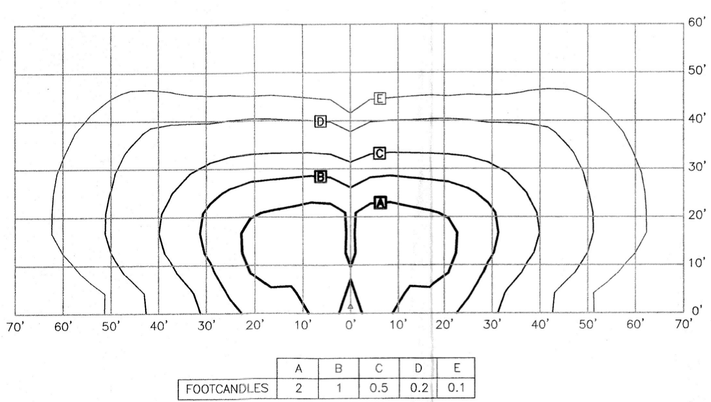
FOOTCANDLE TABLE FOR 69 WATT AREA LIGHTING SCALE: 1"=20'
