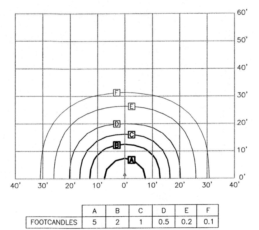
FOOTCANDLE TABLE FOR 56 WATT VACUUM CANOPY LIGHTING SCALE: 1"=20'
