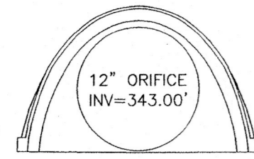
STORMTECH SC-310 CHAMBER INLET END SECTION N.T.S.
