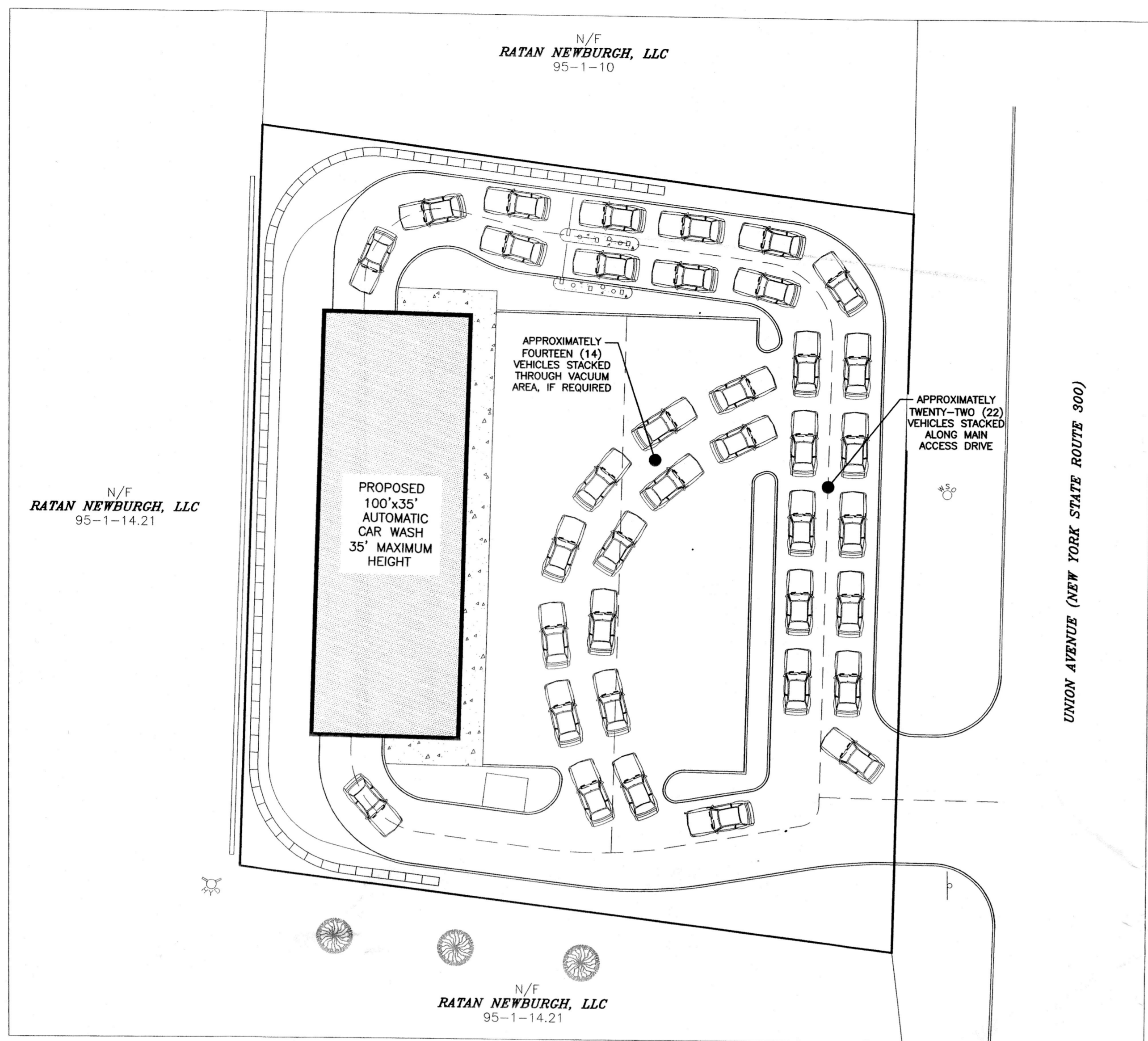
PROPOSED VEHICLE STACKING PLAN
