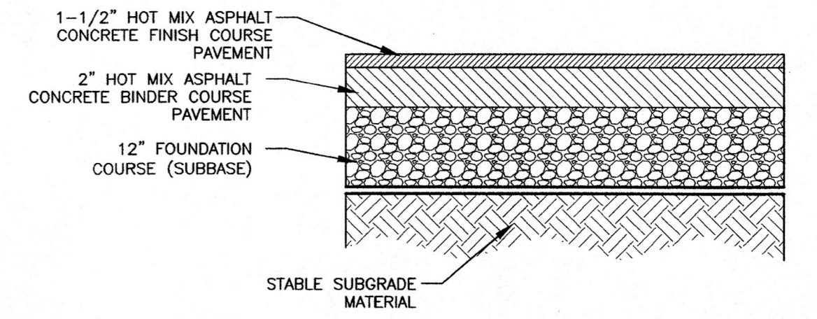
ACCESS DRIVES & PARKING AREA CROSS-SECTION N.T.S.
