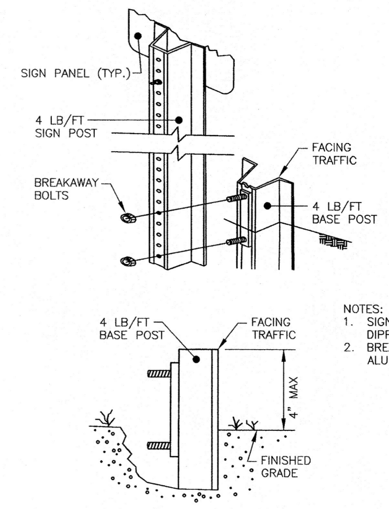
ANCHOR POST ASSEMBLY SIGN SUPPORTS DETAIL N.T.S.
