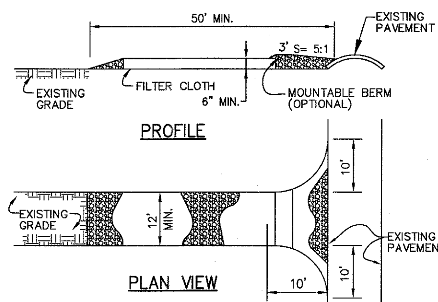
CONSTRUCTION ENTRANCE DETAIL N.T.S.
