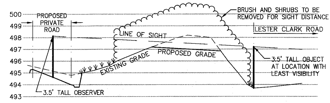
LINE OF SIGHT PROFILE - PRIVATE ROAD ENTRANCE
