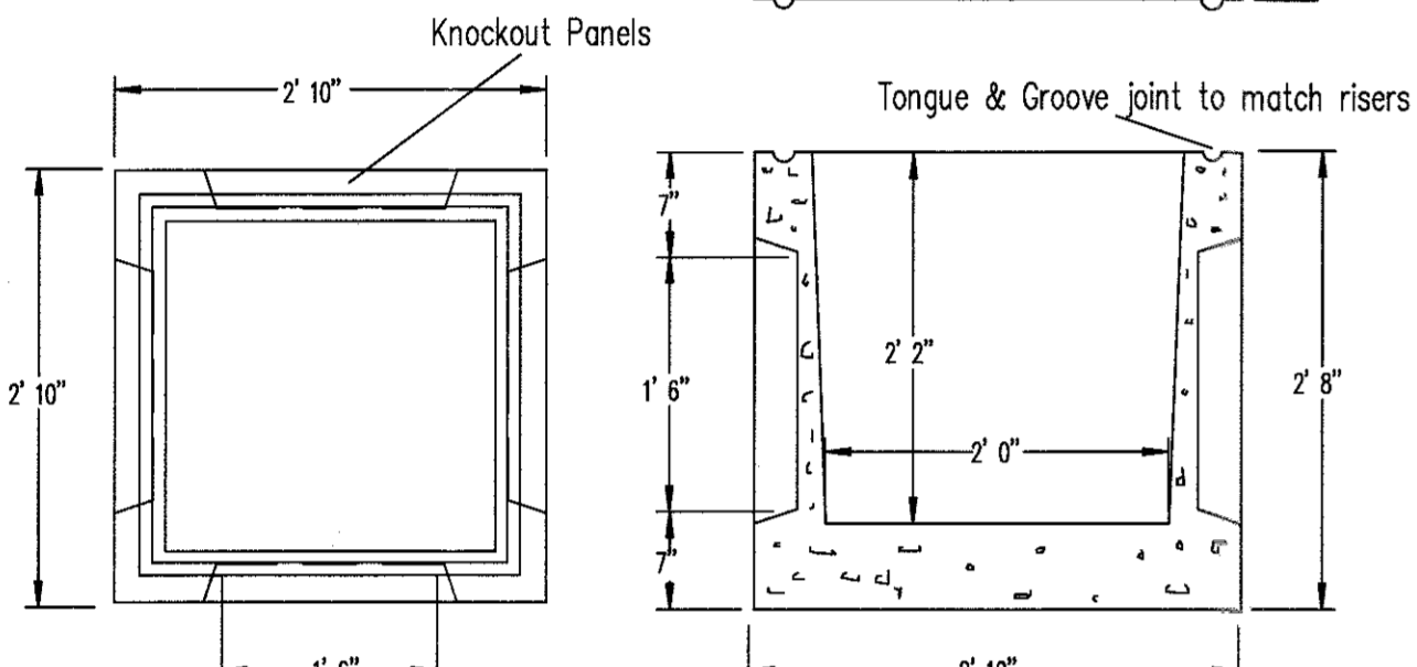
Top View Side View CATCH BASIN TYPE 24x24
