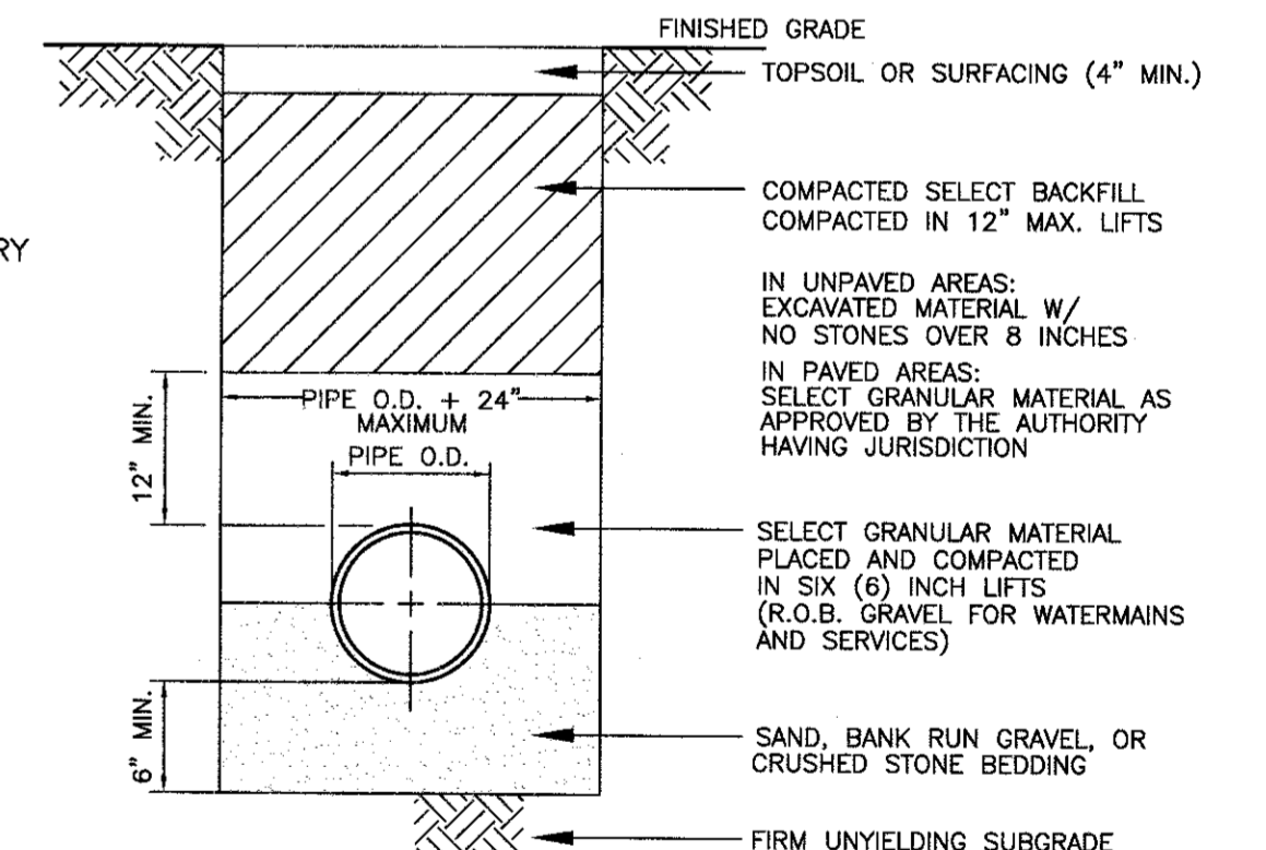
PIPE BEDDING DETAIL (ELSEWHERE)
