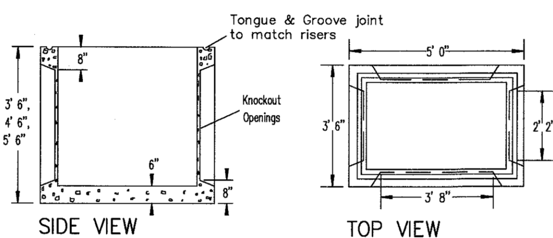
CATCH BASIN TYPE 30x48
