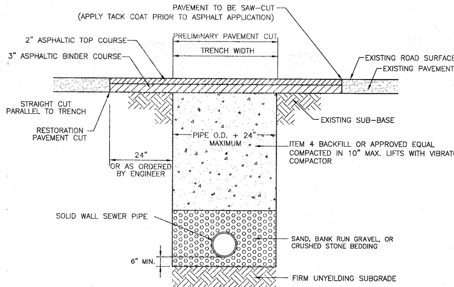
PIPE BEDDING DETAIL (WITHIN LESTER CLARK ROAD)
