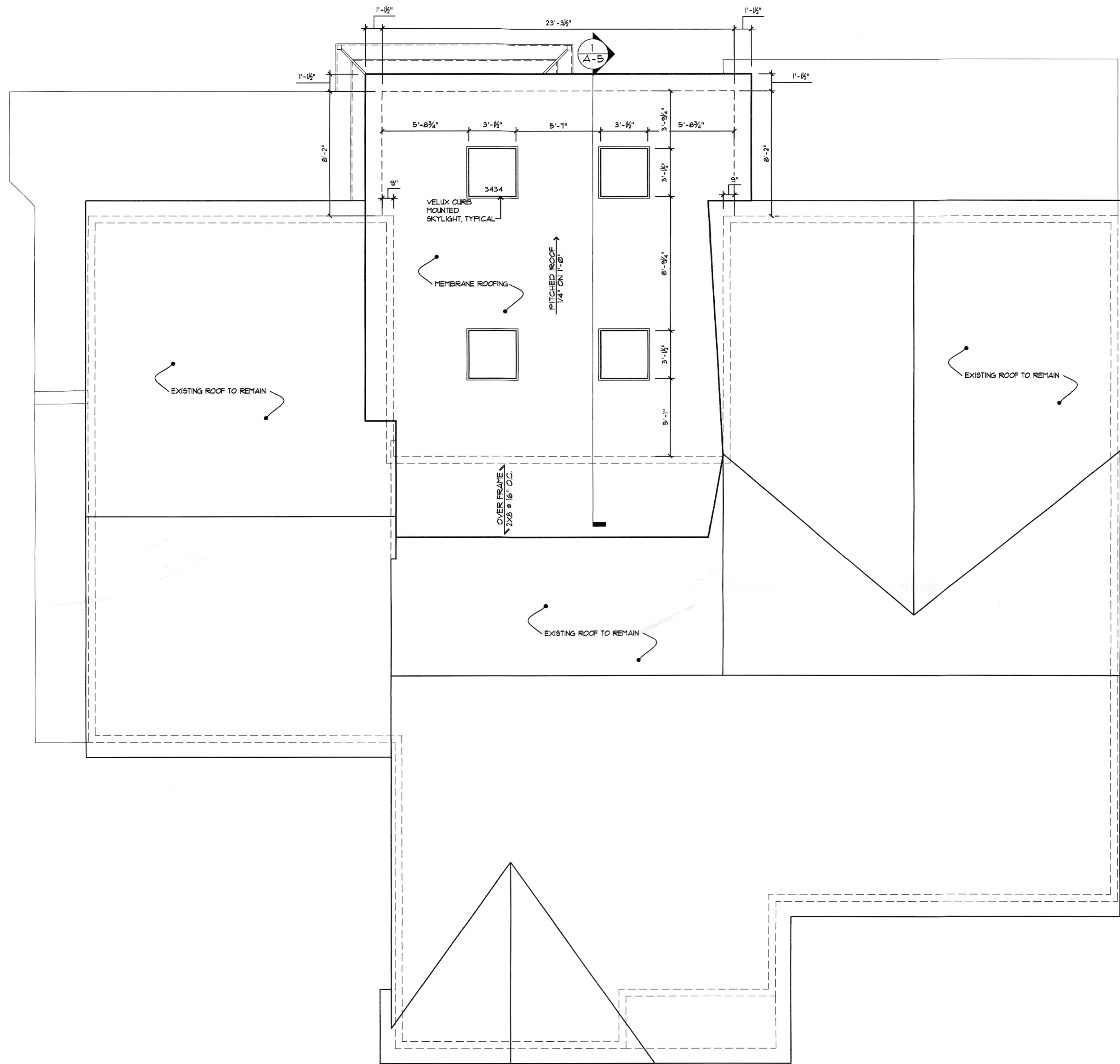
1 PROPOSED ROOF PLAN A-3 SCALE: 1/4" = 1'-0"
