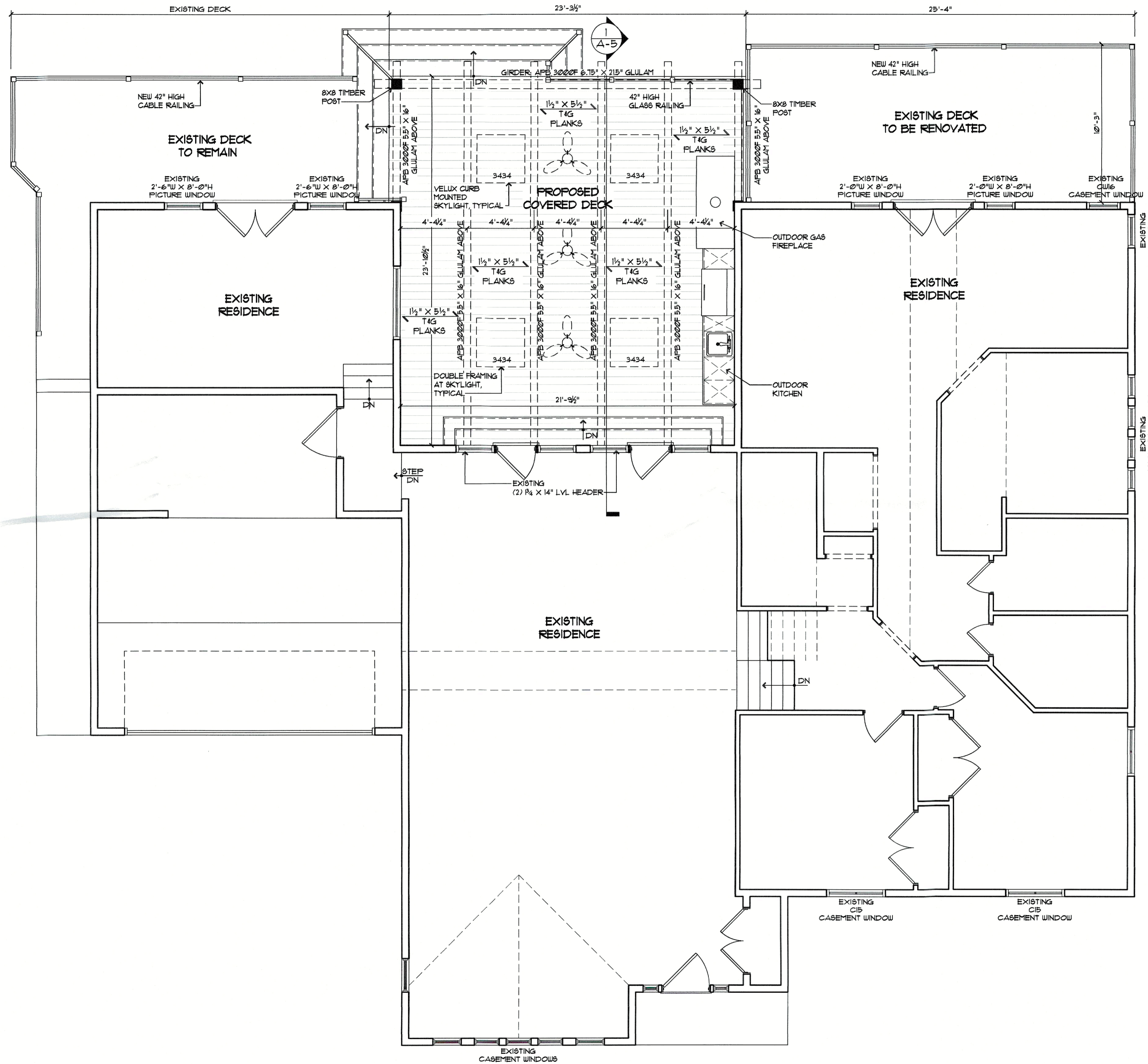
1 PROPOSED FIRST FLOOR PLAN A-2 SCALE: 1/4" = 1'-0"
