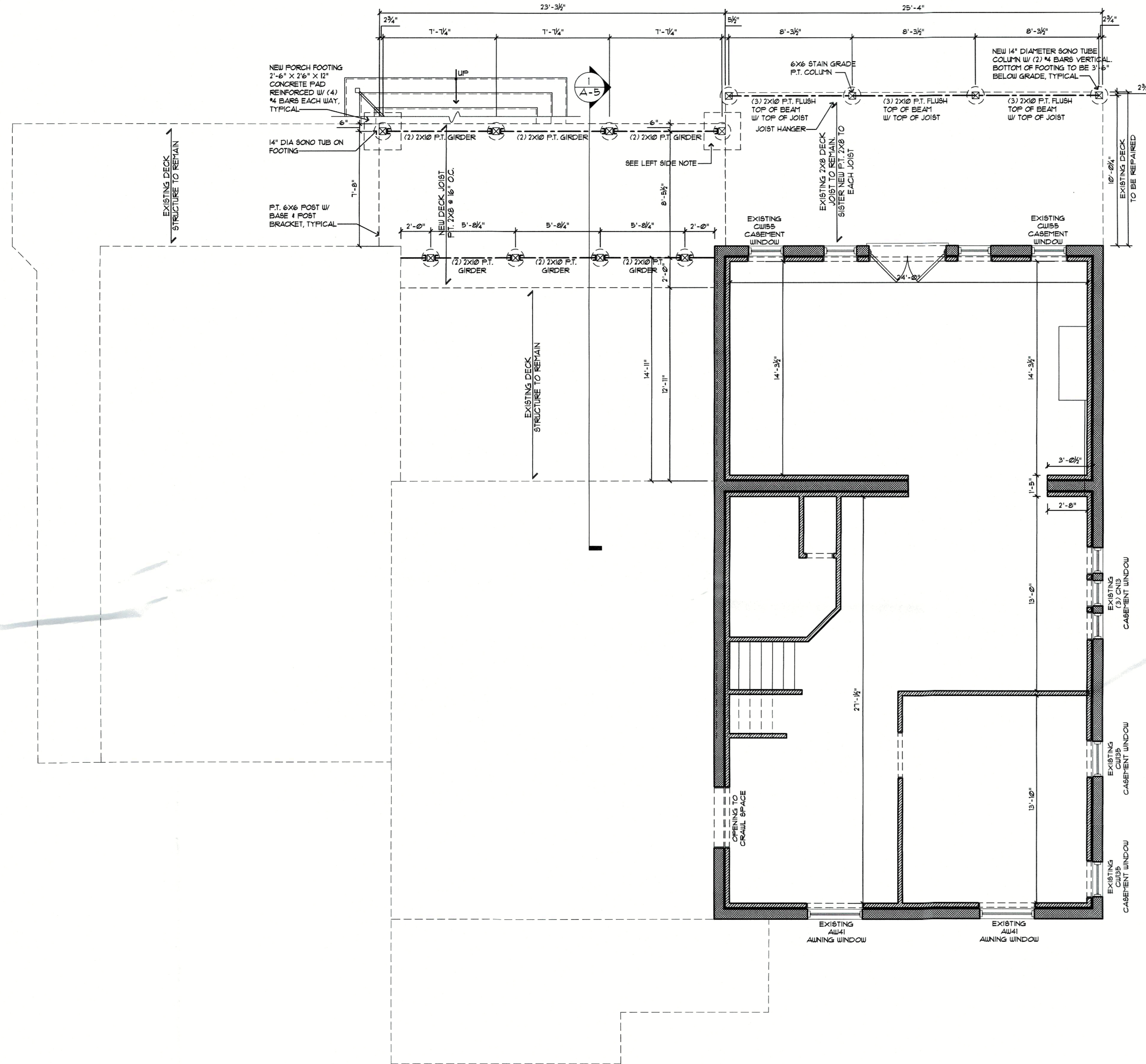
1 PROPOSED FOOTING PLAN A-1 SCALE: 1/4" = 1'-0"
