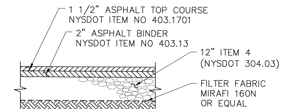
3 PAVEMENT DETAIL SU-1 SCALE: NTS
