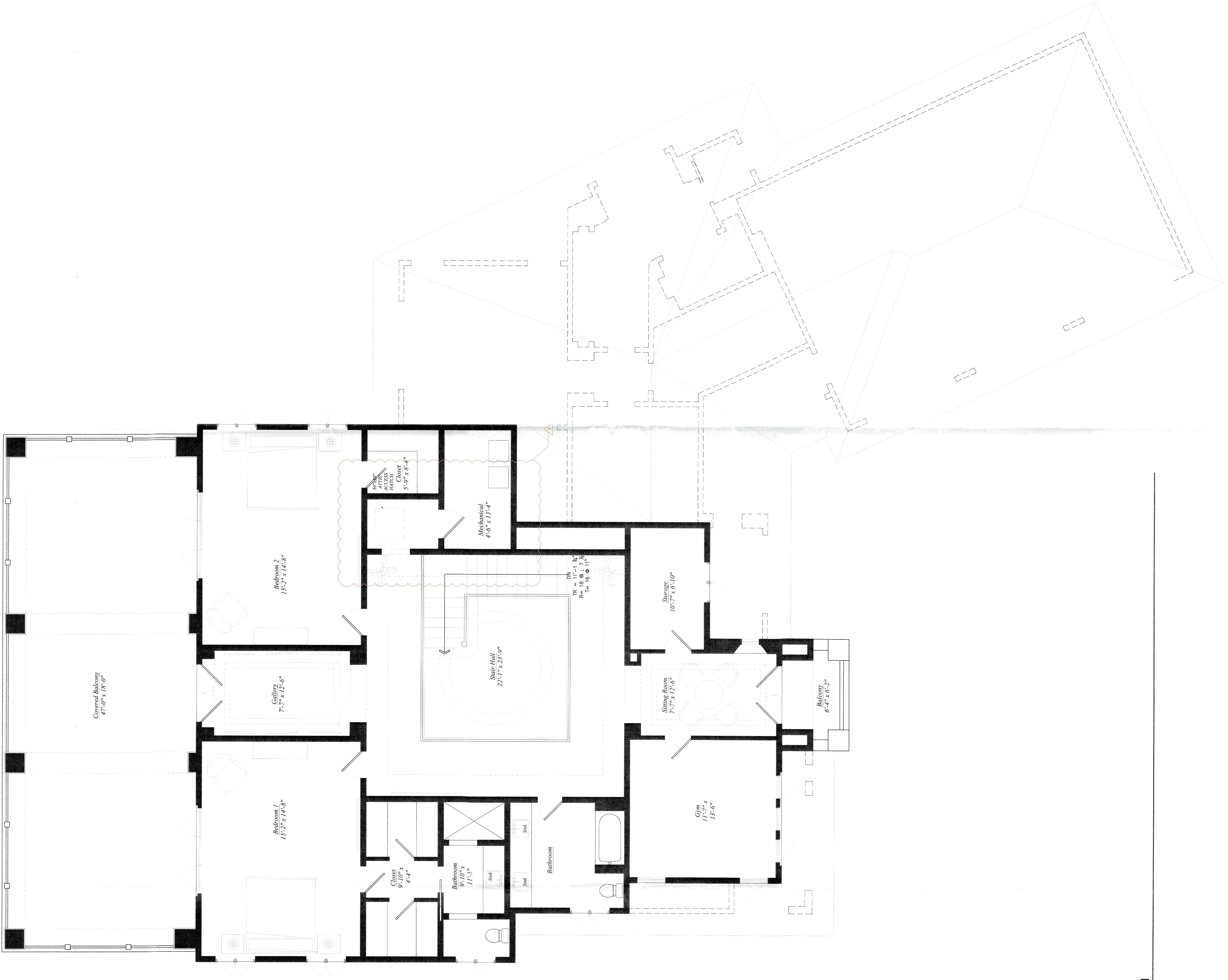
1 Second Floor Architectural A202 Scale: 1/4" = 1'-0"
