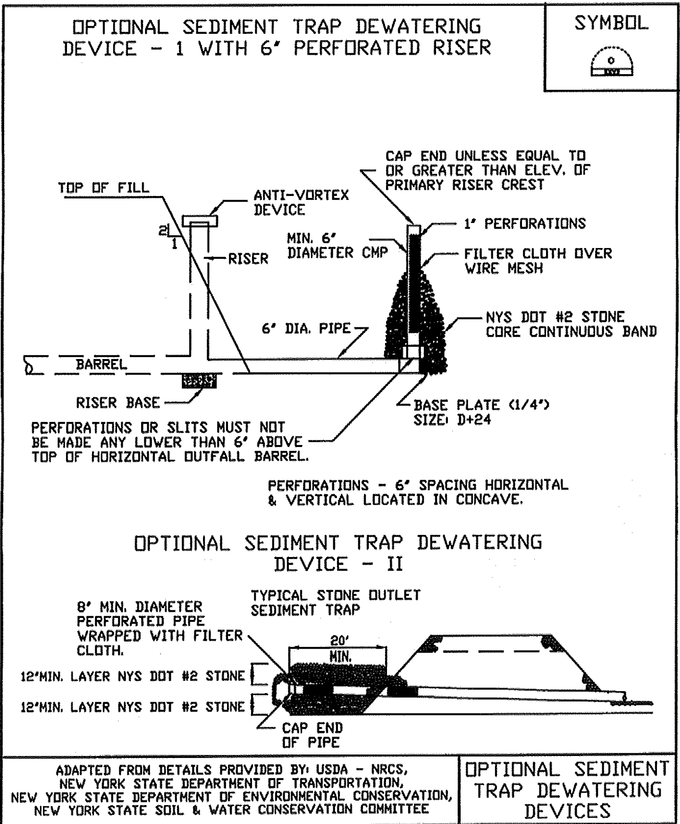
Figure 5A.21 Optional Sediment Trap Dewatering Devices
