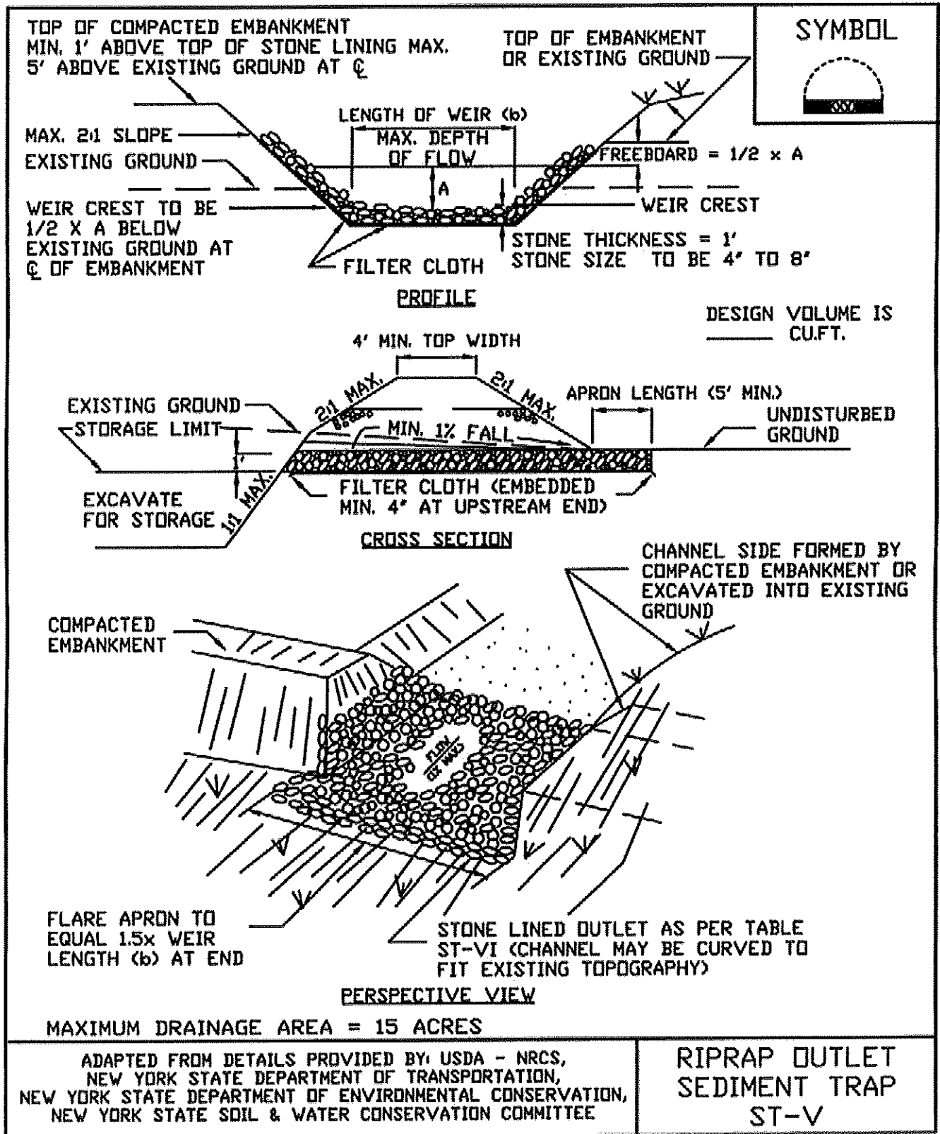
Figure 5A.20(1) Riprap Outlet Sediment Trap: ST-V
