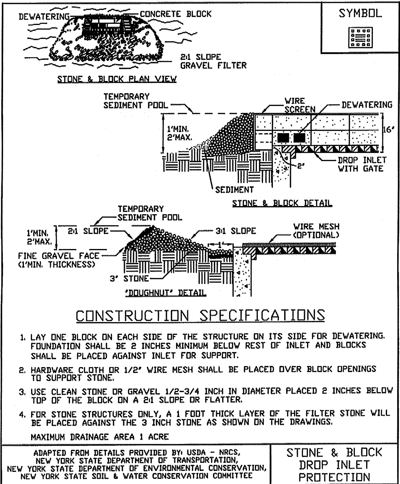
Figure 5A.13 Stone & Block Drop Inlet Protection
