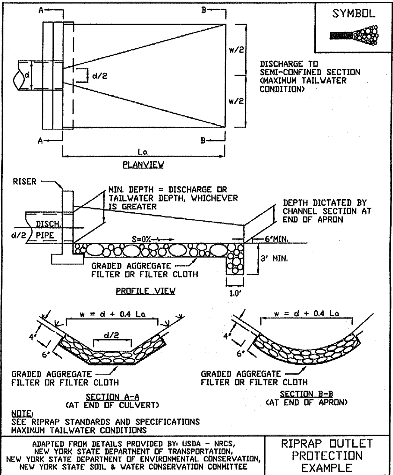
Figure 5B.16 Riprap Outlet Protection Detail (3)
