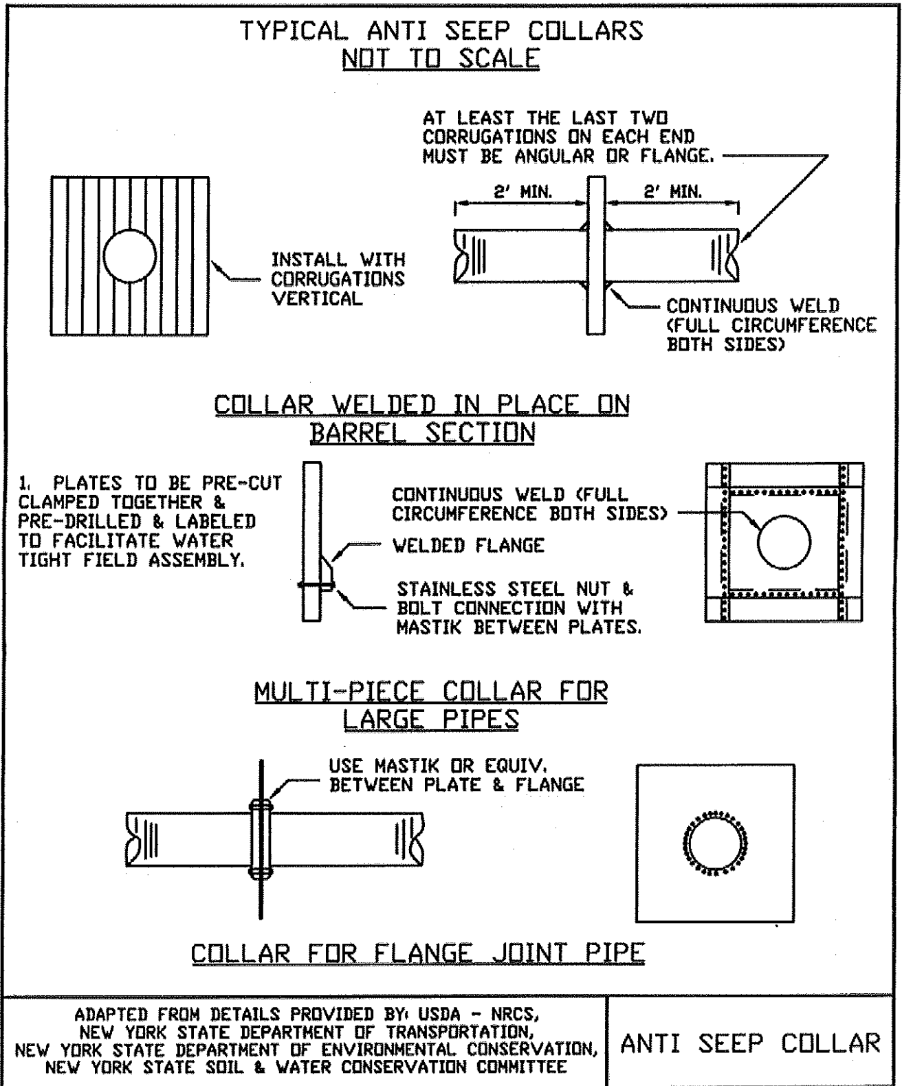
Figure 5A.32 Anti-Seep Collar Design
