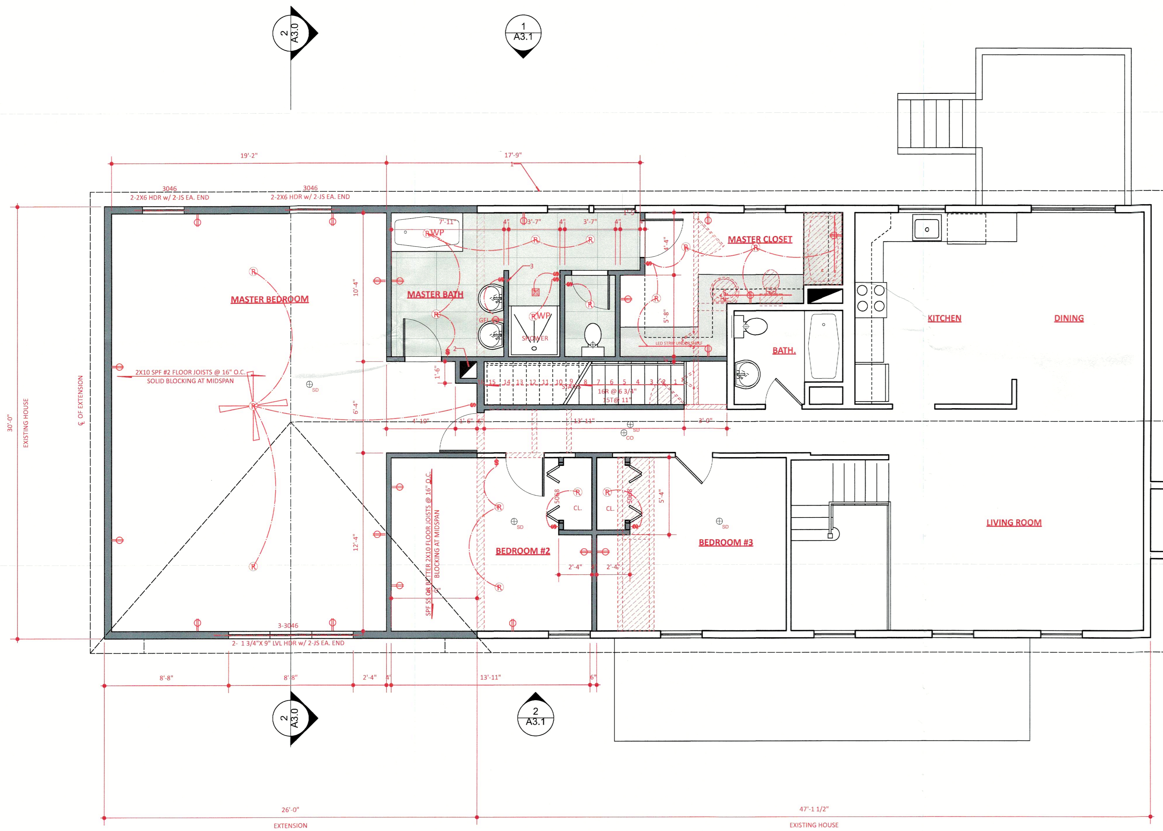
2 FIRST FLOOR PLAN Scale: 1/4" = 1'-0"
