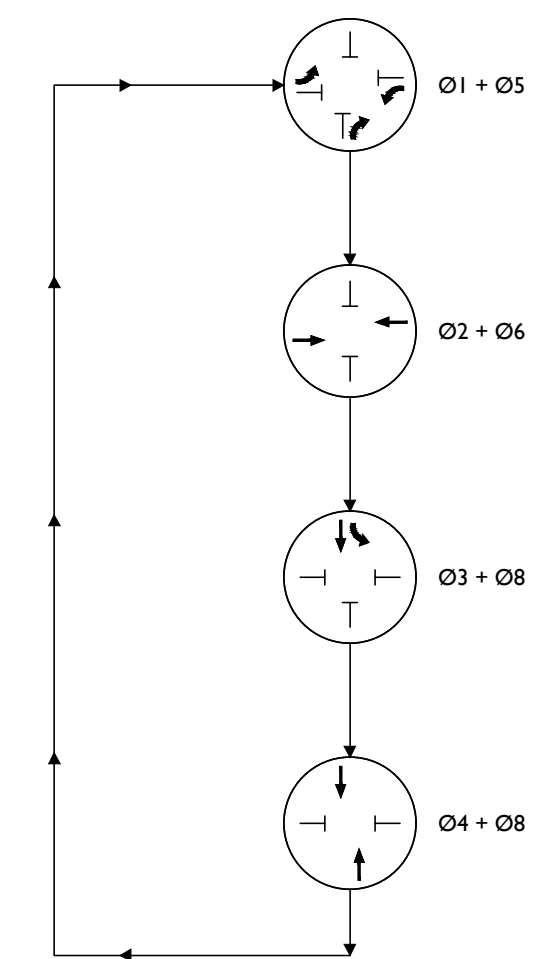
TRAFFIC SIGNAL PHASING DIAGRAM
