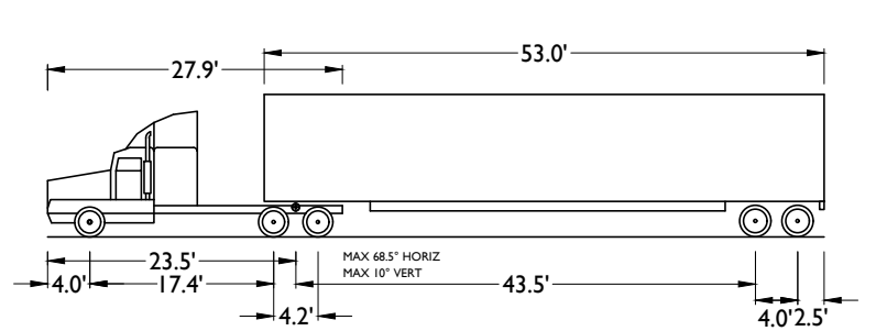
WB-67 - INTERSTATE SEMI-TRAILER
